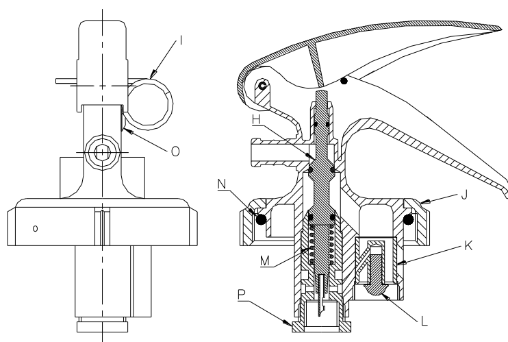
HEADCAP GENERAL ASSEMBLY
